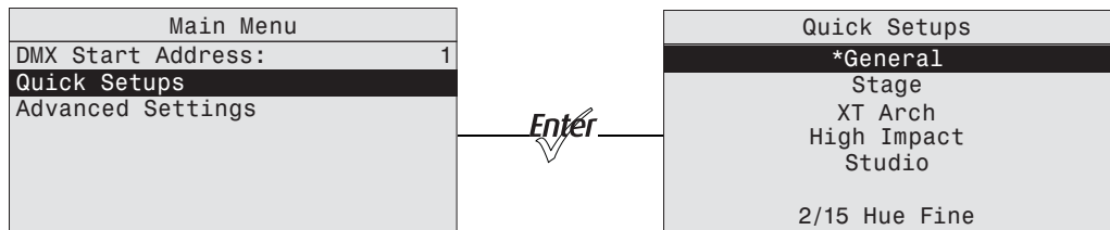
Figure-3.4 Main Menu with Quick Setups selected and the result of pressing Enter. Lustr+ screen shown.
